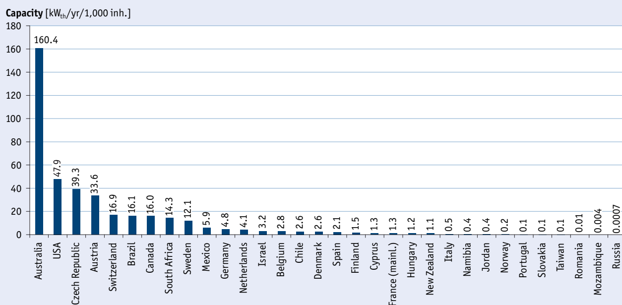
Figure 31: Total capacity of unglazed water collectors in operation in kW th per 1,000 inhabitants in 2016
