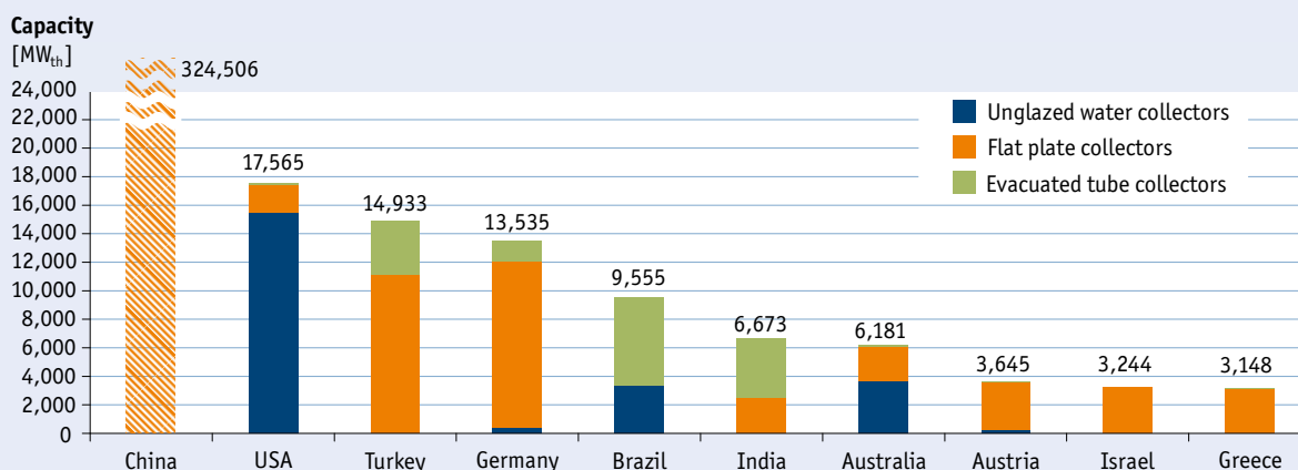
Figure 22: Top 10 countries of cumulated water collector installations (absolute figures in MW th ) 2016
