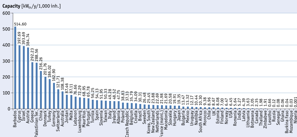
Figure 25: Total capacity of glazed water collectors in operation in kW th per 1,000 inhabitants in 2016
