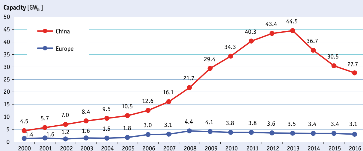
Figure 42: Market development of glazed water collectors in China and Europe 2000 – 2016
