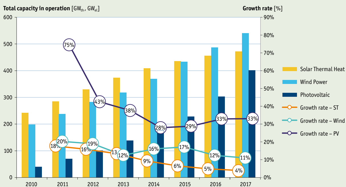
Figure 4: Global capacity in operation and market growth rates between 2010 and 2017 (Sources: AEE INTEC, Global Wind Energy Council (GWEC), SolarPower Europe, REN21 – Global Status Reports 2011 – 2018)
