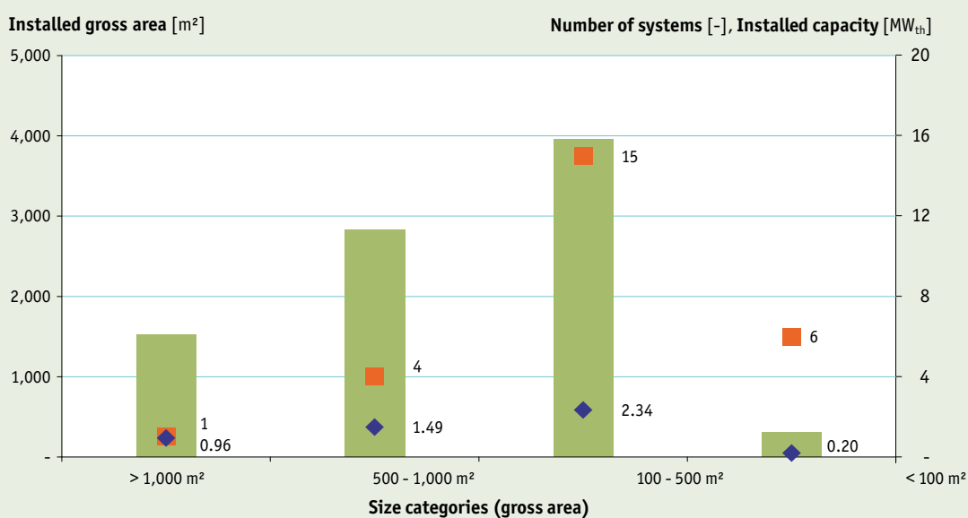
Figure 12: Number, gross area and thermal capacity of installed plants with concentrating collector types in different size categories in India by end of March 2018. (Source: IEA SHC Task49 / IV SHIP database)
