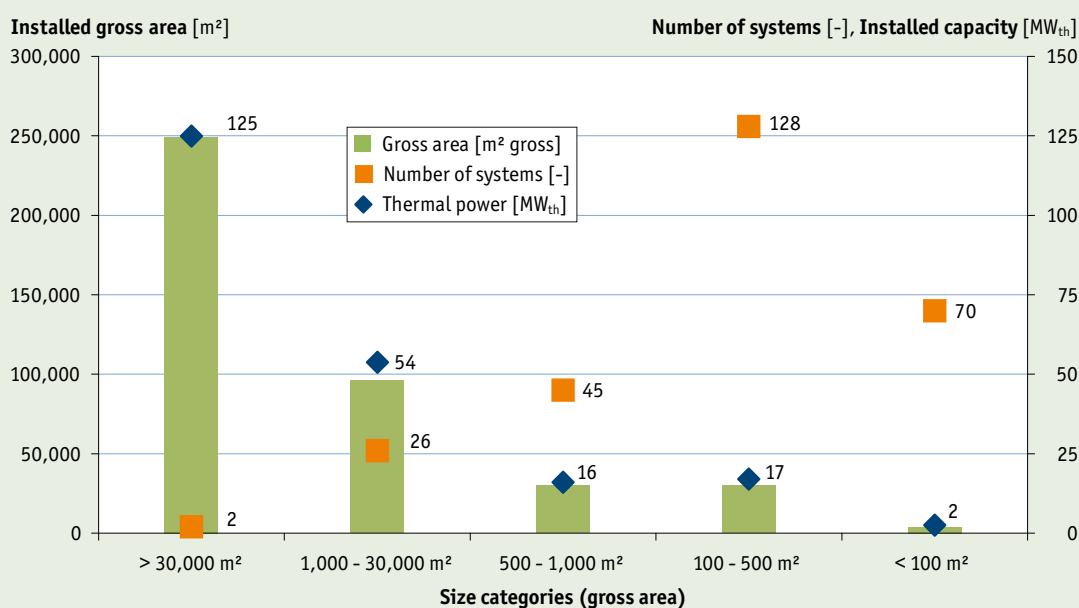
Figure 13: Global solar process heat plants in operation by capacity and collector area by end of March 2018 (Source: IEA SHC Task49 / IV SHIP database)
