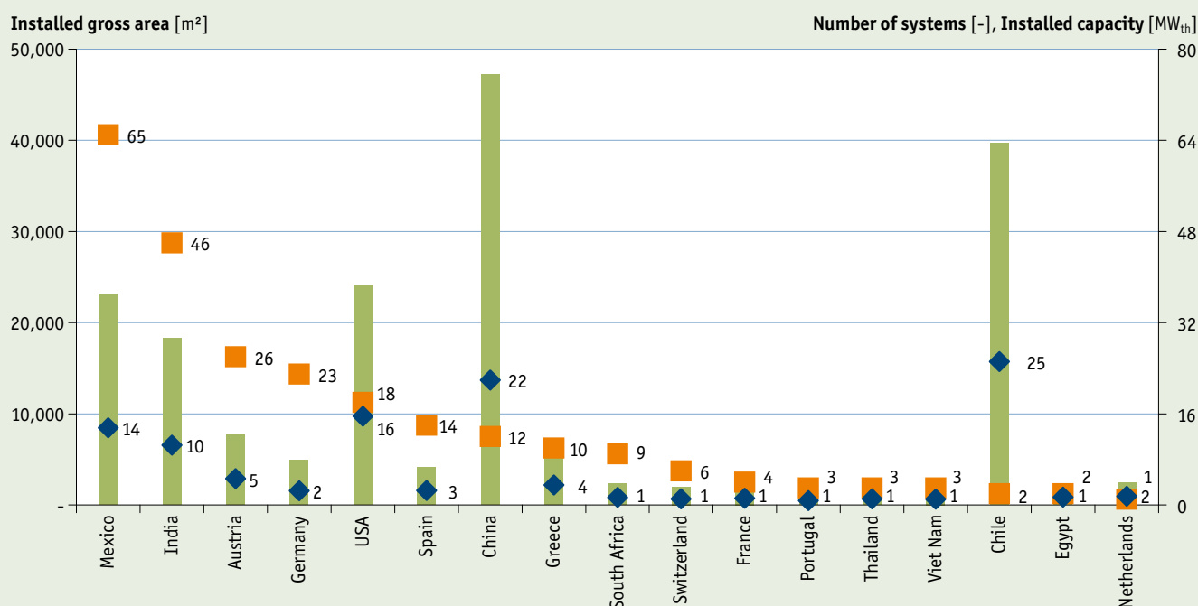
Figure 16: Global solar process heat installations in operation by country by end of March 2018. Only countries with at least 0.7 MW th (1,000 m² gross area) are shown (248 of 271 systems accounting for 98% of installed thermal capacity) (Source: IEA SHC Task49 / IV SHIP database)
