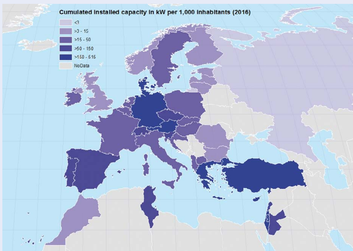
Figure 27: Solar thermal market penetration per capita in Europe in \text{kW}_{\text{th}} per 1,000 inhabitants
