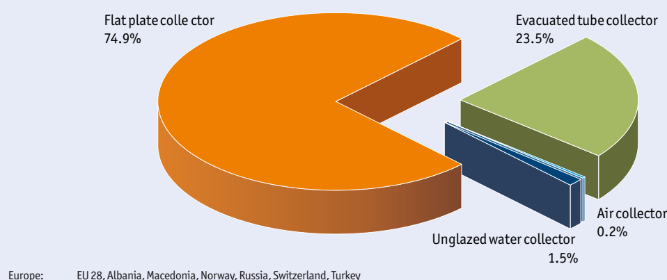
Figure 34: Distribution of the newly installed capacity by collector type in 2016 – EUROPE
