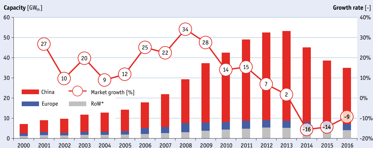
Figure 41: Global market development of glazed water collectors from 2000 to 2016
