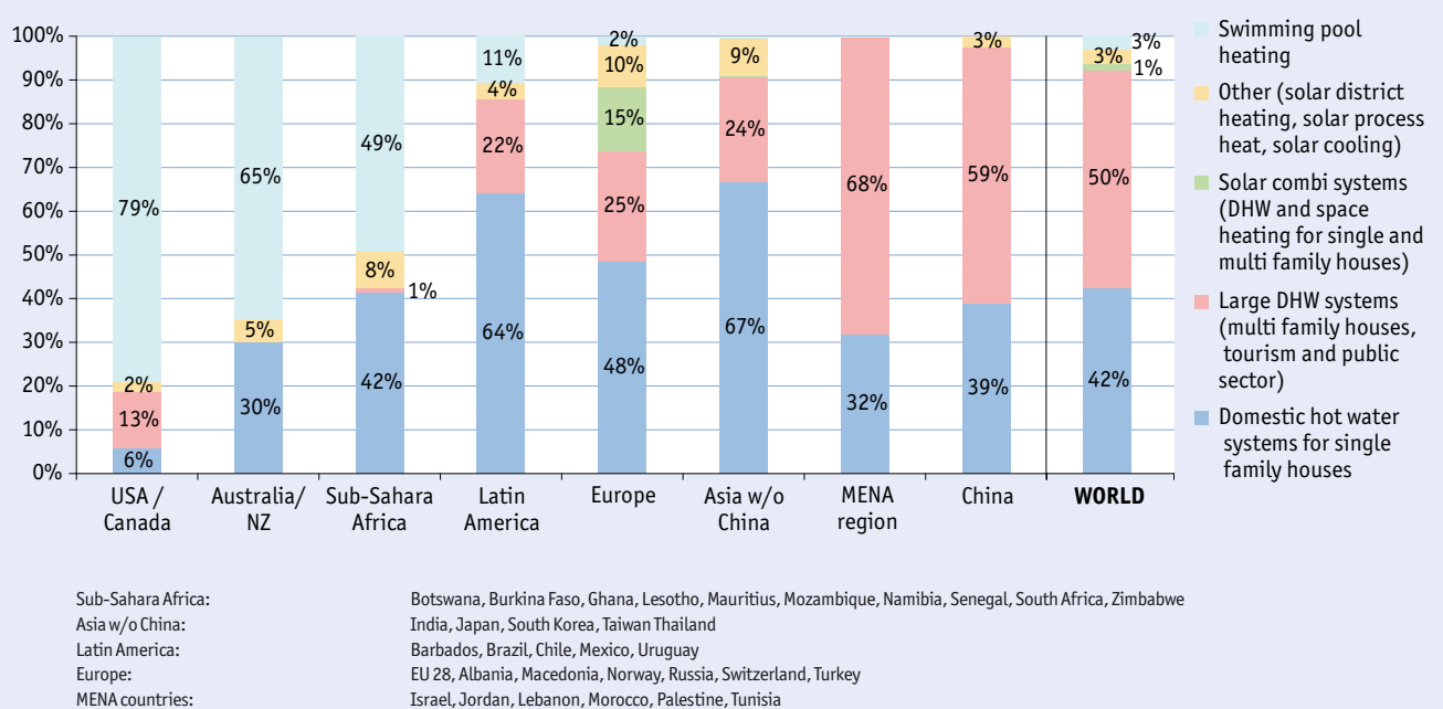
Figure 56: Distribution of solar thermal systems by application for the newly installed water collector capacity by economic region in 2016
