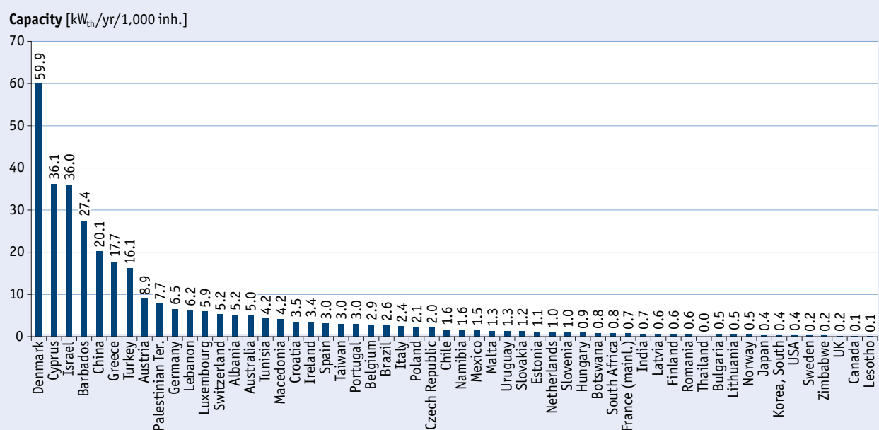
Figure 38: Newly installed capacity of glazed water collectors in 2016 in kW th per 1,000 inhabitants
