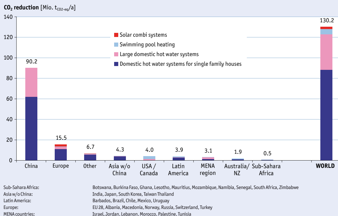
Figure 50: Contribution to CO 2 reduction by unglazed and glazed water collectors in operation in 2016
