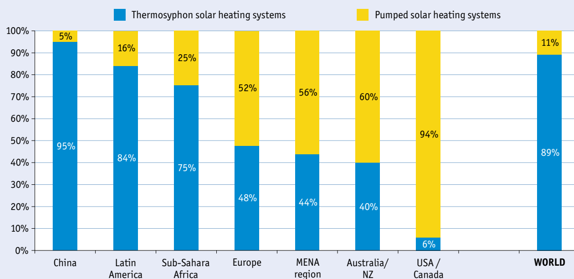
Figure 53: Distribution by type of system for the total installed glazed water collector capacity in operation by the end of 2016
