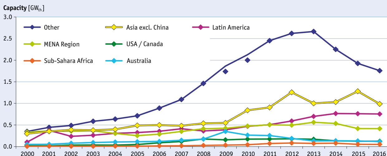
Figure 44: Market development of glazed water collectors in Rest of World (excluding China and Europe) from 2000 to 2016
