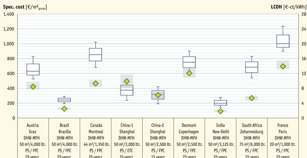
Figure 60: Specific investment costs and levelized costs of solar thermal generated heat for large pumped domestic hot water systems
