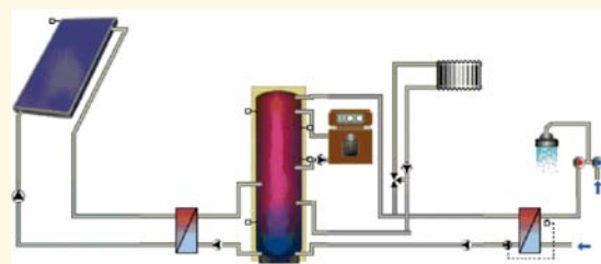
Hydraulic scheme of the solar-combi reference system for single and multifamily houses
