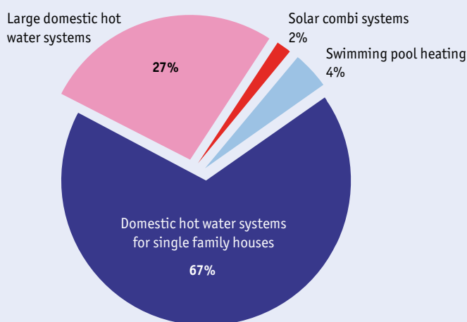
Figure 47: Share of energy savings and CO 2 reduction by type of application of glazed and unglazed water collectors in operation in 2016
