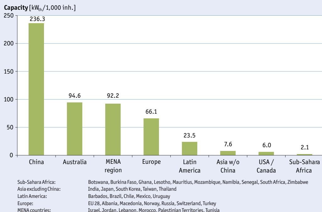
Figure 29: Total capacity of glazed flat plate and evacuated tube collectors in operation by economic region and in \text{kW}_{\text{th}} per 1,000 inhabitants in 2016
