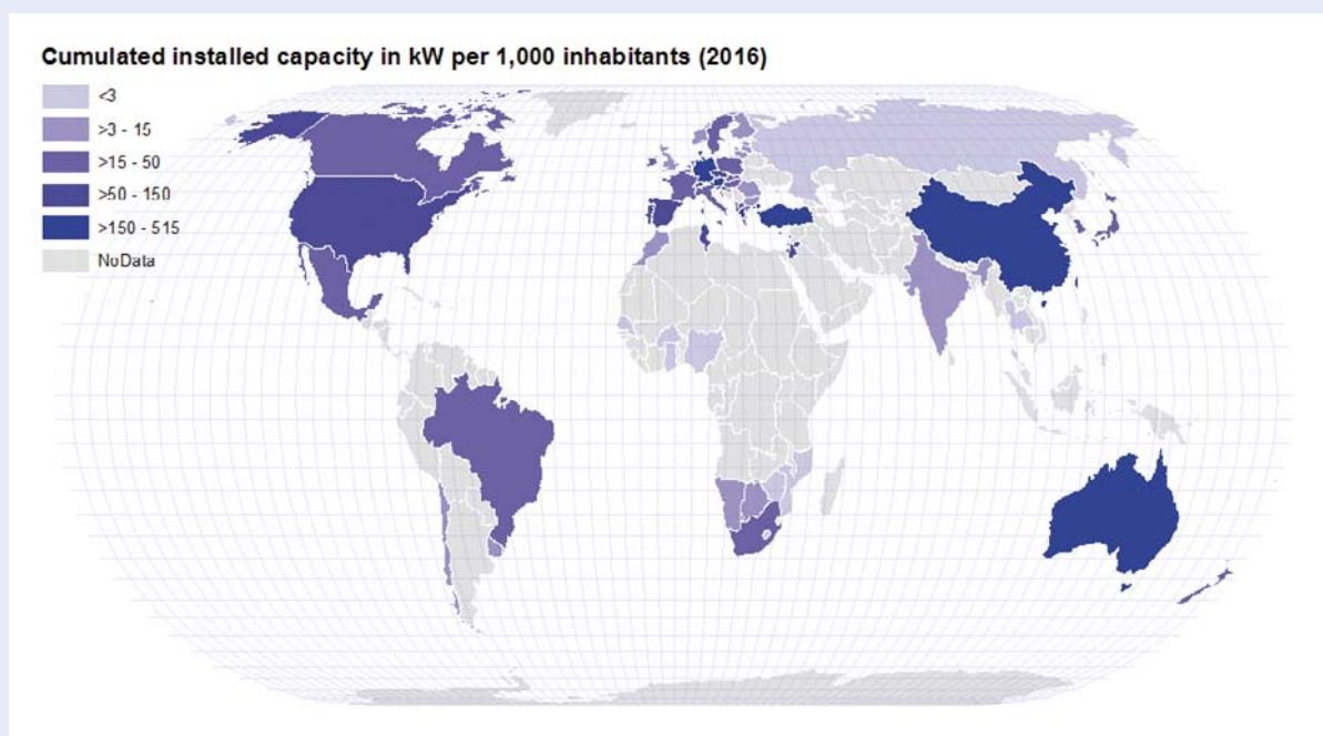
Figure 26: Solar thermal market penetration per capita worldwide in \text{kW}_{\text{th}} per 1,000 inhabitants
