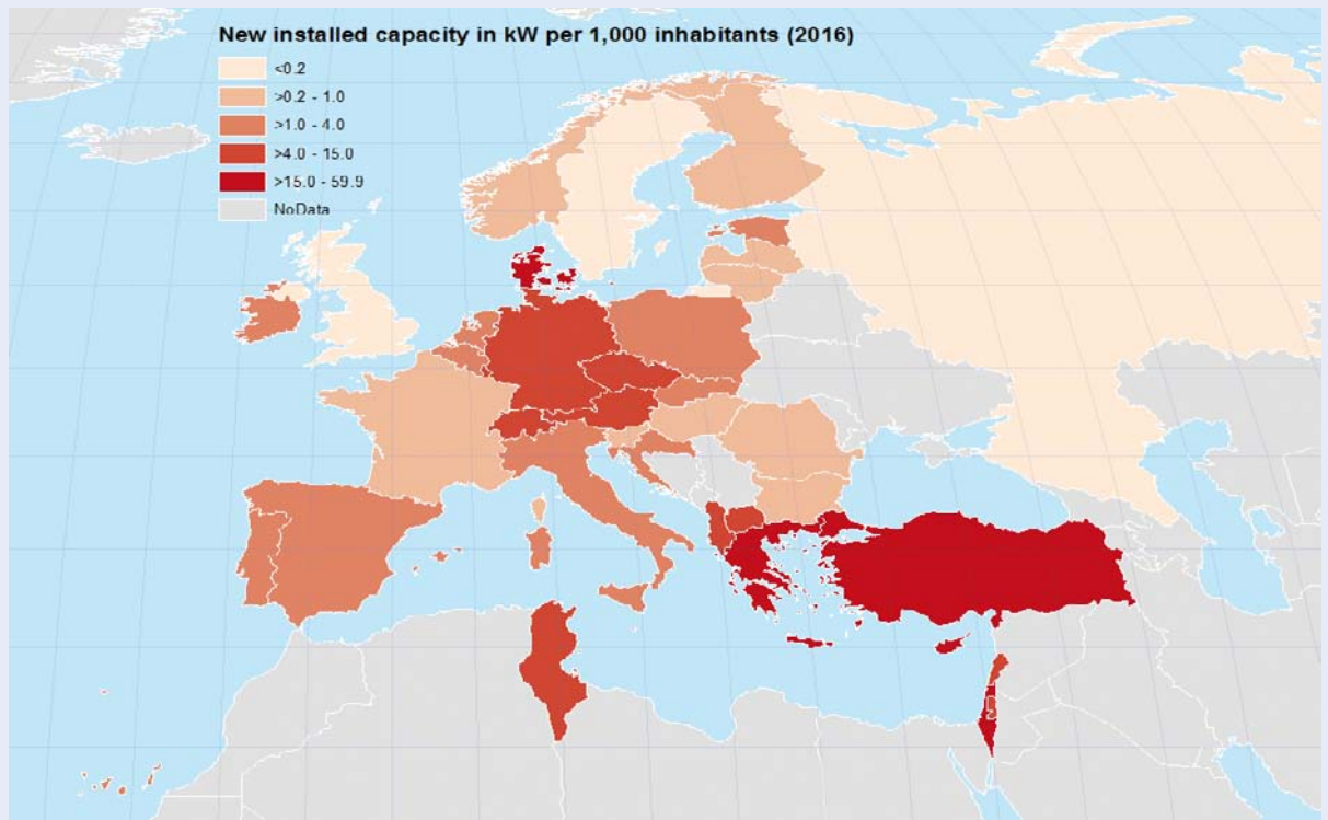
Figure 39: Installed capacity in Europe in 2016 in \text{kW}_{\text{th}} per 1,000 inhabitants
