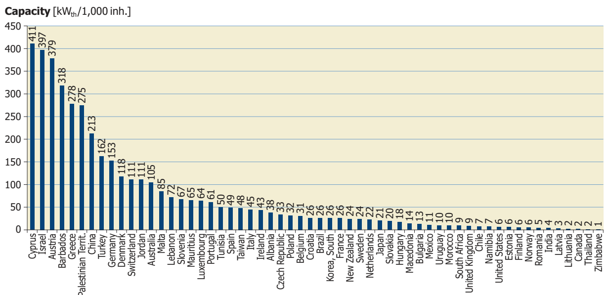
Figure 11: Total capacity of glazed water collectors in operation in kW th per 1,000 inhabitants in 2014
