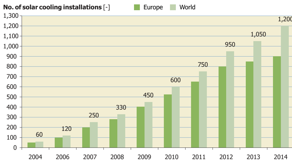
Figure 42: Market development 2004 – 2014 of small to large-scale solar air conditioning and cooling systems (Source: Solem Consulting, Tecsol)
