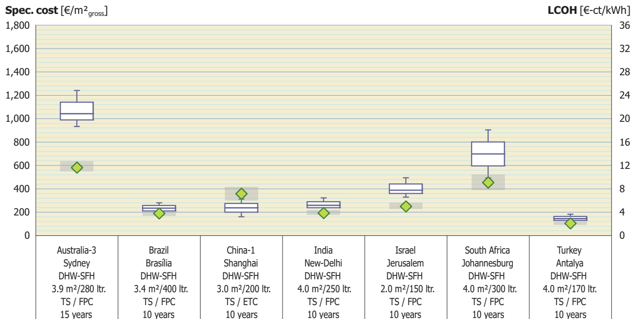
Figure 45: Specific Investment costs and levelized costs of solar thermal generated heat for small thermosiphon domestic hot water systems
