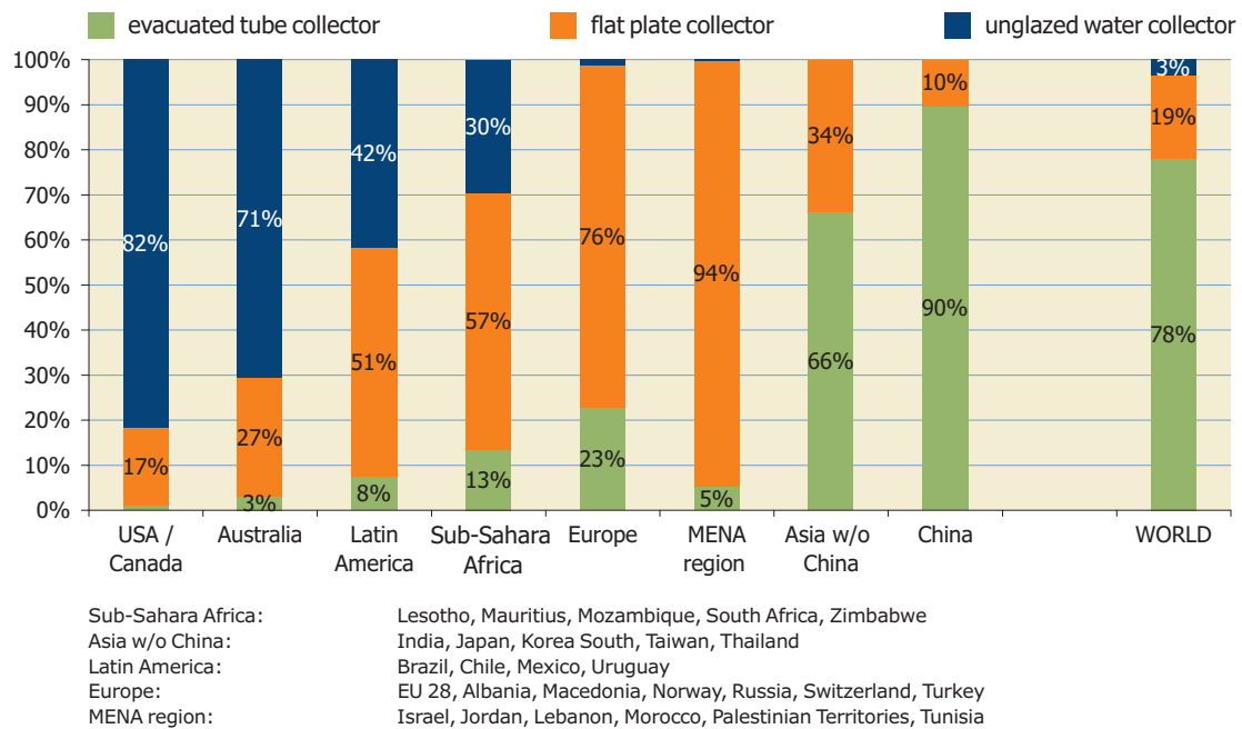
Figure 35: Distribution by type of solar thermal collector for the new installed water collector capacity in 2014
