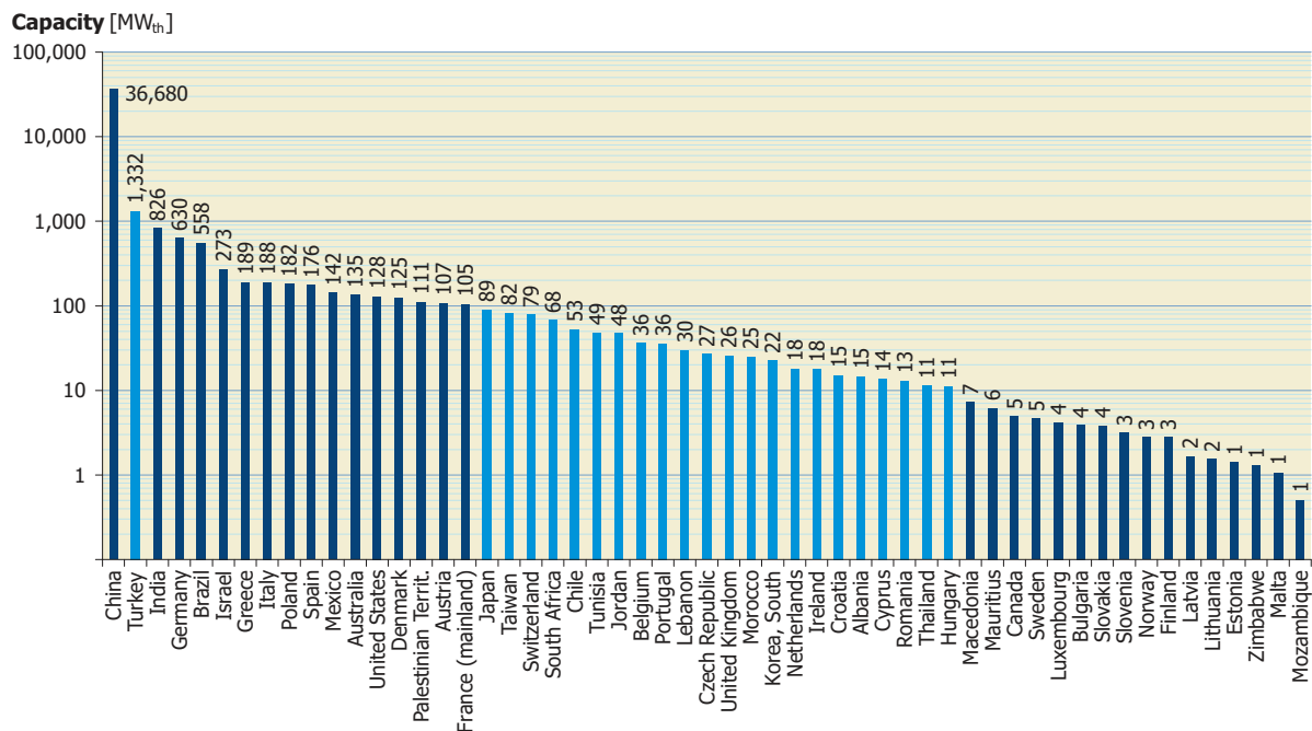
Figure 22: New installed capacity of glazed water collectors in 2014
