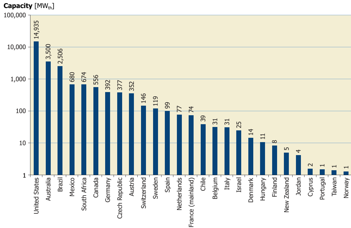
Figure 14: Total capacity of unglazed water collectors in operation in 2014
