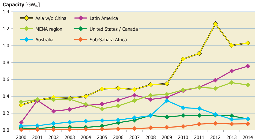
Figure 27: Market development of glazed water collectors in Rest of World (w/o China and Europe) from 2000 to 2014
