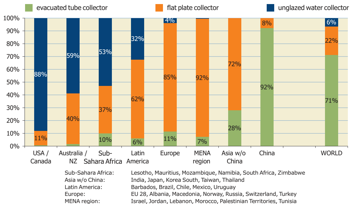
Figure 34: Distribution by type of solar thermal collector for the total installed water collector capacity in operation by the end of 2014
