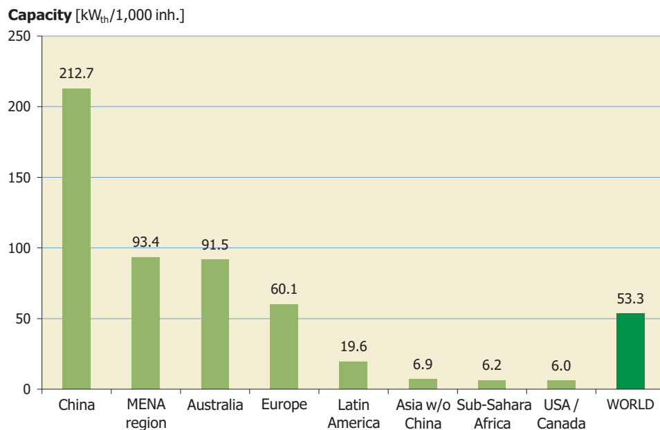
Figure 13: Total capacity of glazed flat plate and evacuated tube collectors in operation by economic region and in kW th per 1,000 inhabitants in 2014
