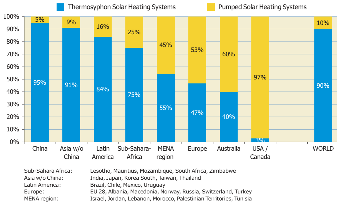
Figure 37: Distribution by type of system for the new installed glazed water collector capacity in 2014
