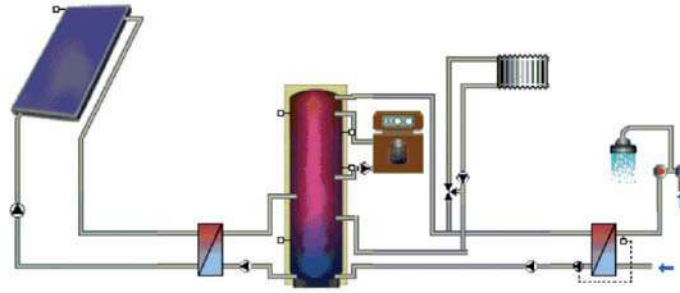
Figure 53: Hydraulic scheme of the solar-combi reference system for single and multifamily houses
