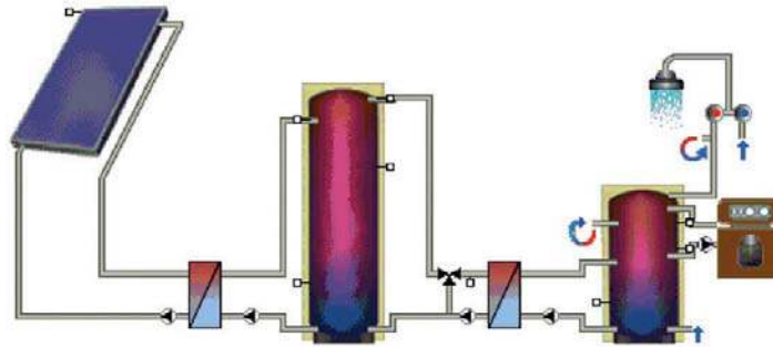
Figure 52: Hydraulic scheme of the domestic hot water pumped reference system for multifamily houses
