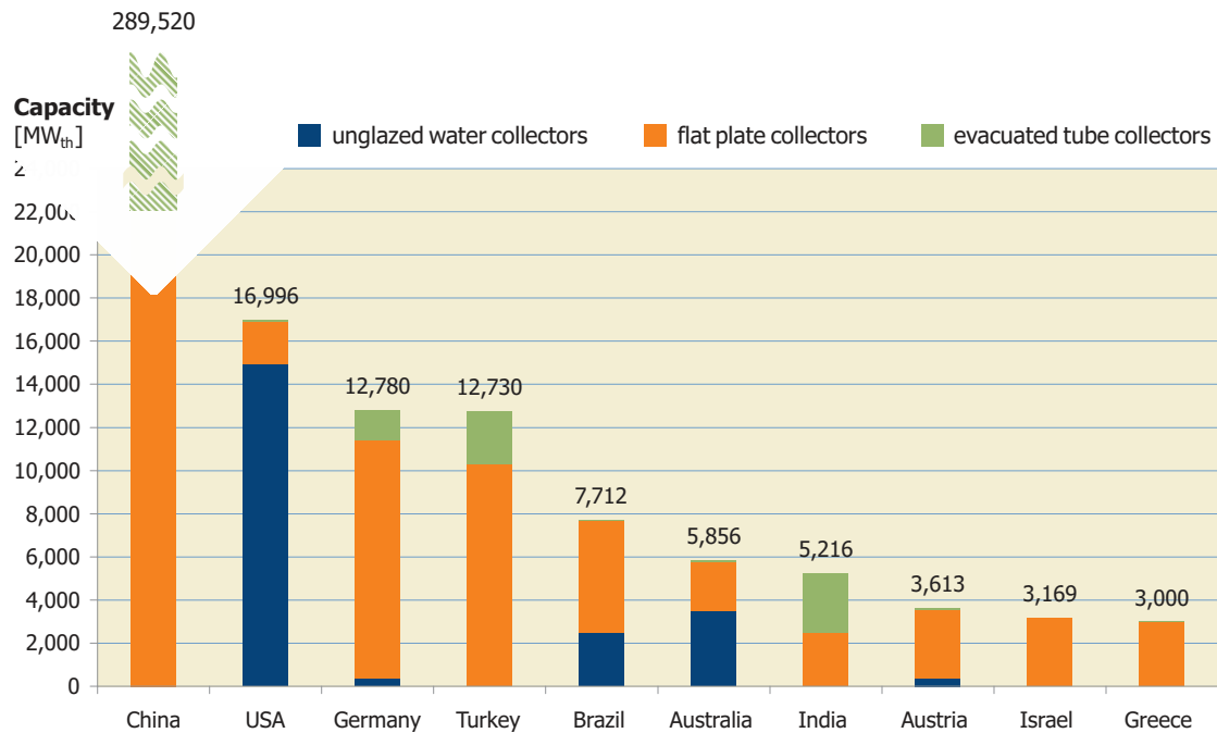
Figure 8: Top 10 countries of cumulated water collector installations (absolute figures in MW th )
