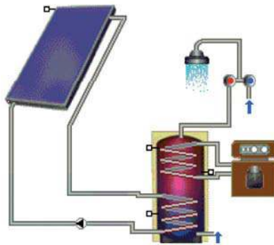
Figure 50: Hydraulic scheme of the domestic hot water pumped reference system for single-family houses
