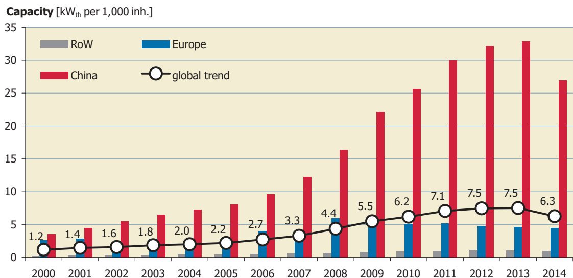
Figure 28: Annual installed capacity of glazed water collectors in kW th per 1,000 inhabitants from 2000 to 2014
