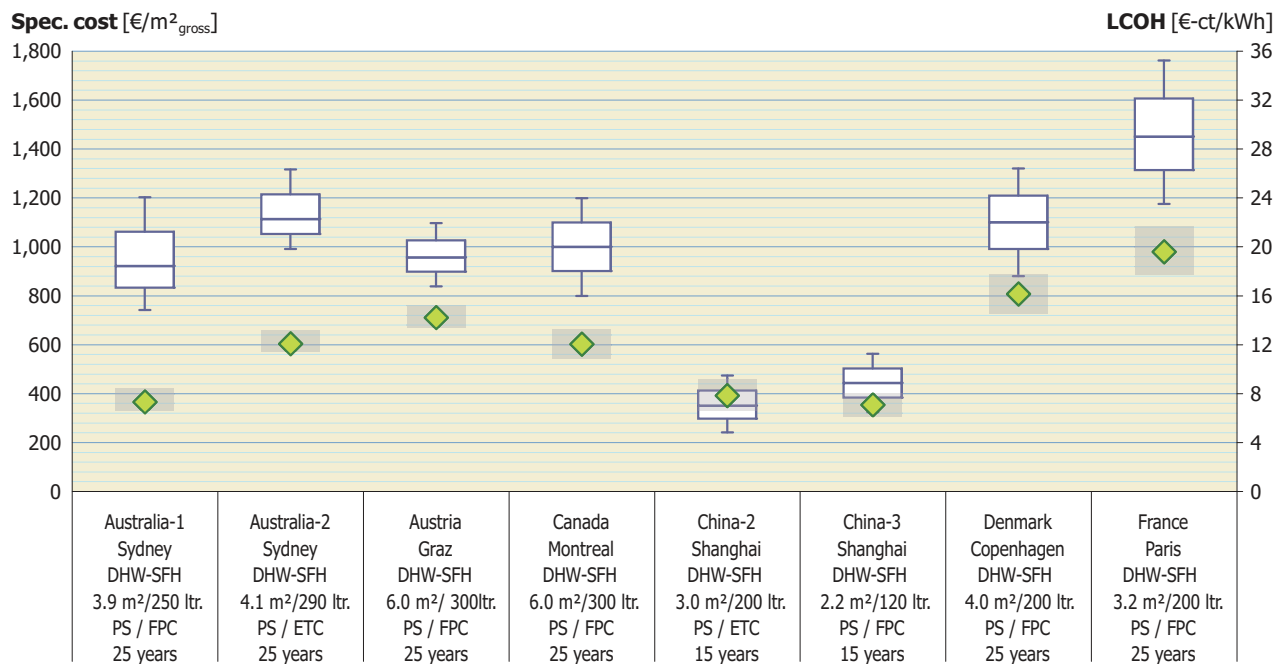
Figure 44: Specific Investment costs and levelized costs of solar thermal generated heat for small pumped domestic hot water systems
