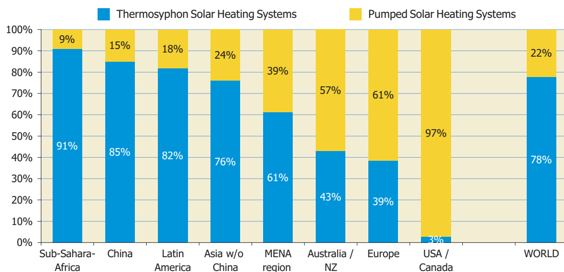
Figure 36: Distribution by type of system for the total installed glazed water collector capacity in operation by the end of 2014
