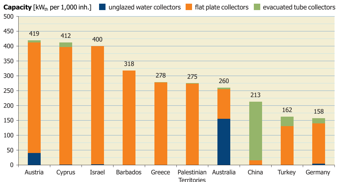
Figure 9: Top 10 countries of cumulated water collector installations (relative figures in kW th per 1,000 inhabitants)
