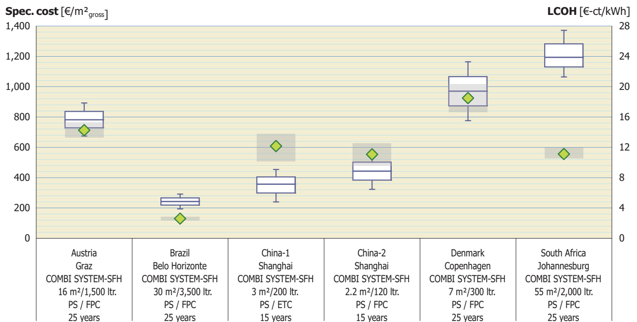
Figure 47: Specific Investment costs and levelized costs of solar thermal generated heat for small combined hot water and space heating systems
