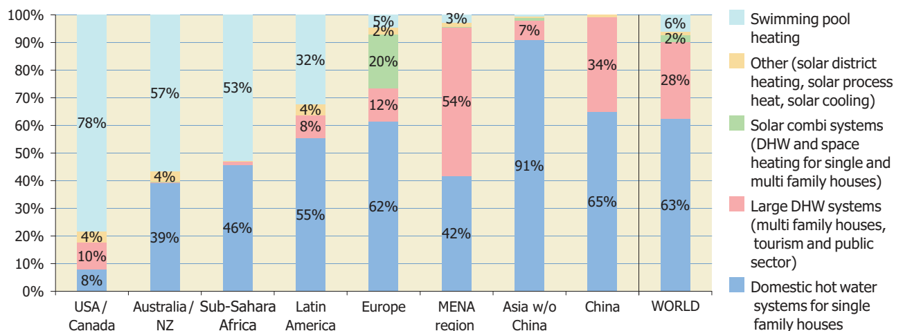
Figure 38: Distribution of solar thermal systems by application for the total installed water collector capacity by economic region in operation by the end of 2014
