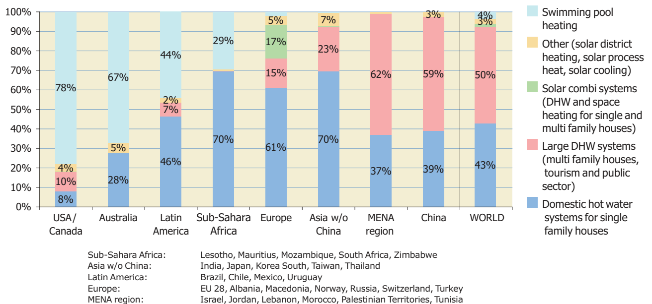
Figure 39: Distribution of solar thermal systems by application for the new installed water collector capacity by economic region in 2014
