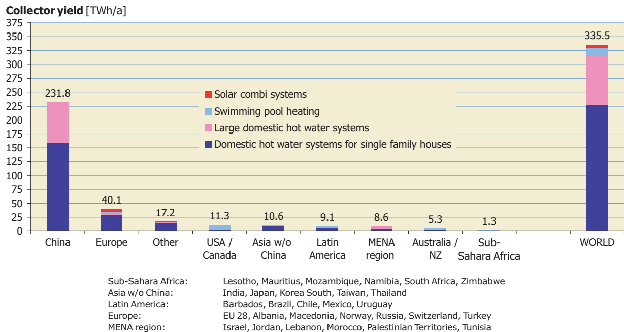
Figure 31: Annual collector yield of unglazed and glazed water collectors in operation in 2014
