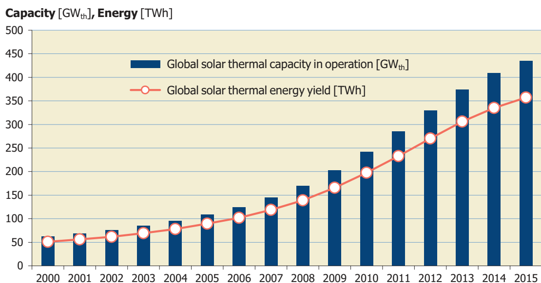
Figure 2: Global solar thermal capacity in operation and annual energy yields 2000–2015
