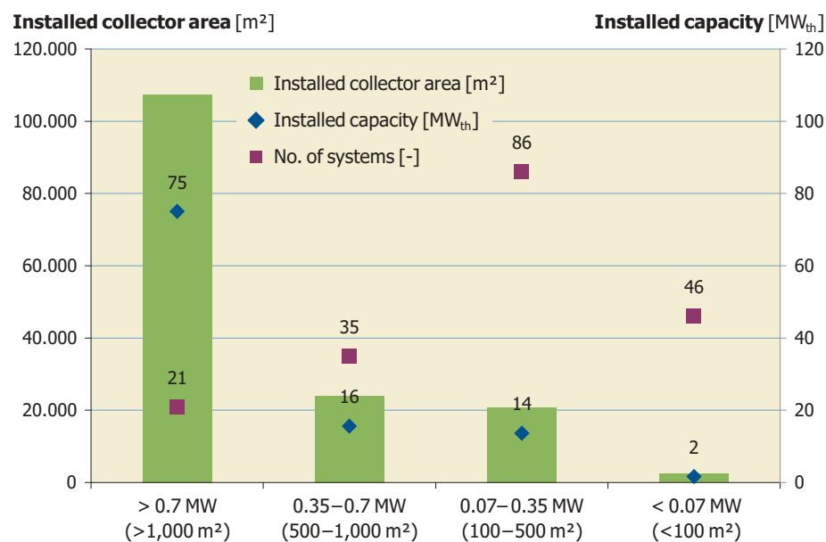
Figure 43: Global solar process heat applications in operation by April 2016 (Source: IEA SHC Task49/IV SHIP database)
