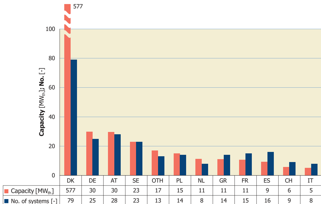
Figure 41: Solar district heating and cooling in Europe – capacities installed and No. of systems in 2015 (Data source: Jan-Olof Dalenbäck – Chalmers University of Technology, SE)
