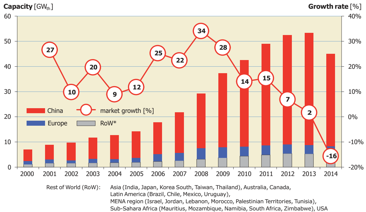
Figure 24: Global market development of glazed water collectors from 2000 to 2014
