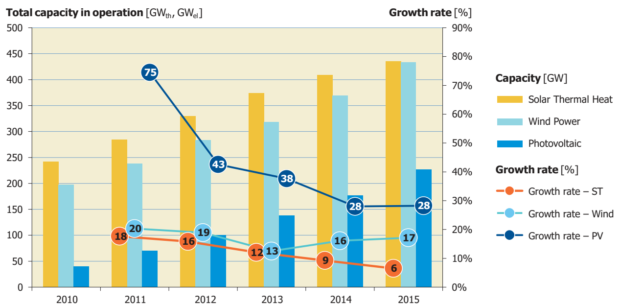
Figure 4: Global solar thermal heat, wind power and photovoltaic capacity in operation and market growth rates between 2010 and 2015 (Sources: AEE INTEC, Global Wind Energy Council (GWECC), European PV Industry Association (EPIA), REN21 - Global Status Reports 2011-2015)
