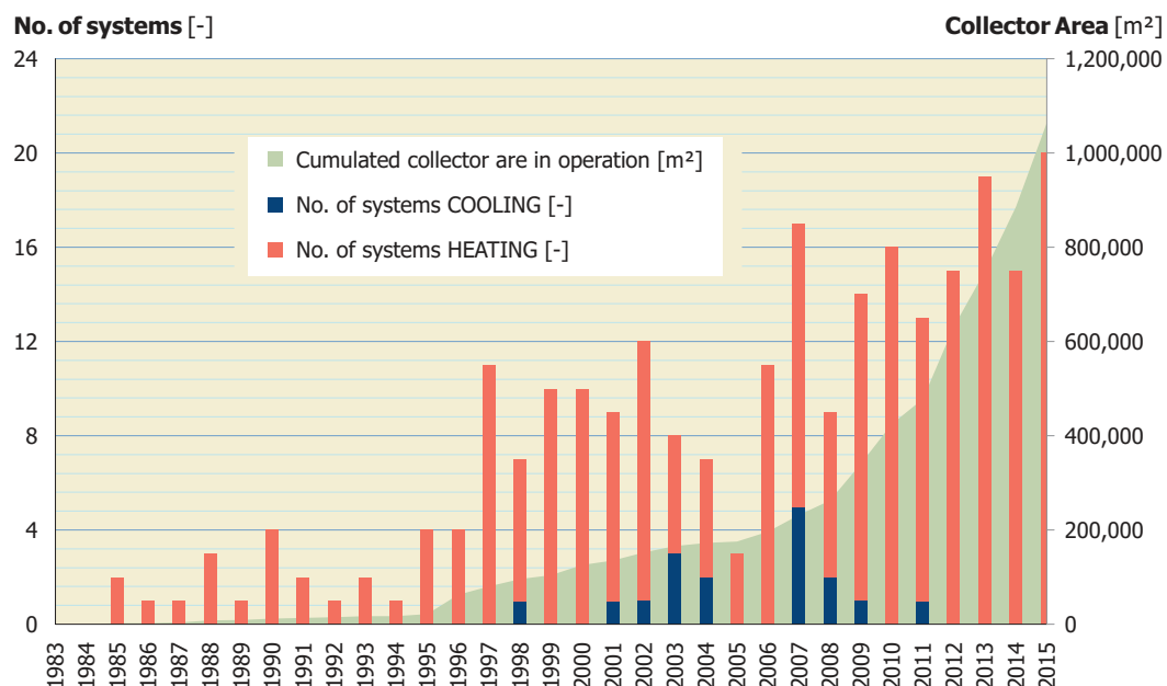
Figure 40: Solar district heating and cooling in Europe – annual achievements and cumulated area in operation in 2015 (Data source: Jan-Olof Dalenbäck – Chalmers University of Technology, SE)
