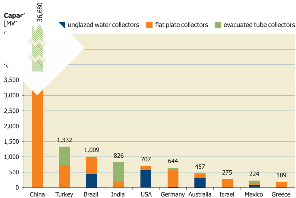
Figure 20: Top 10 markets for glazed and unglazed water collectors in 2014 (absolute figures in MW th )
