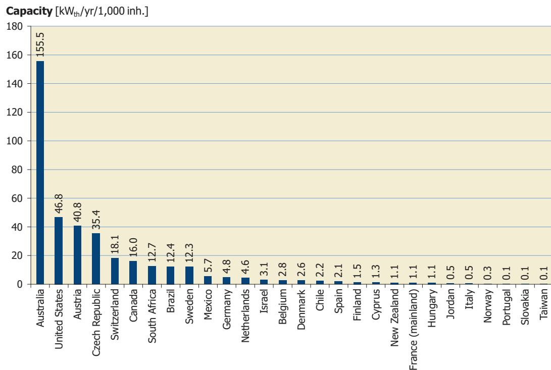
Figure 15: Total capacity of unglazed water collectors in operation in kW th per 1,000 inhabitants in 2014
