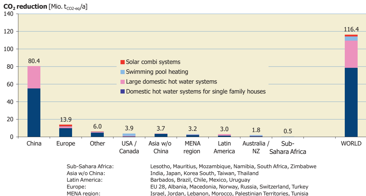
Figure 33: Contribution to CO 2 reduction by unglazed and glazed water collectors in operation in 2014
