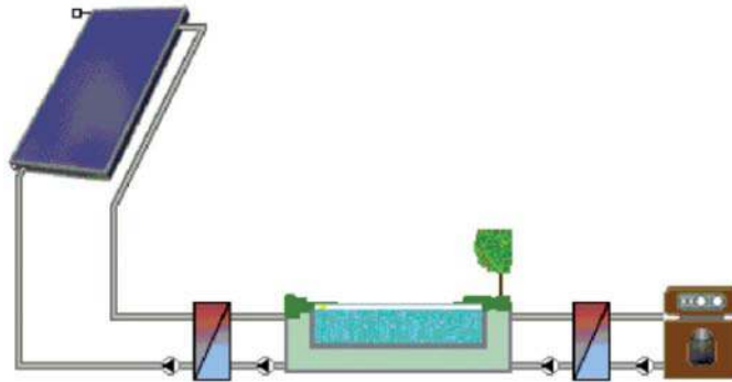
Figure 49: Hydraulic scheme of the swimming pool reference system
