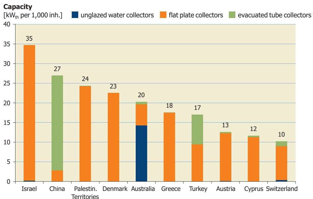
Figure 21: Top 10 markets for glazed and unglazed water collectors in 2014 (relative figures in kW th per 1,000 inhabitants)
