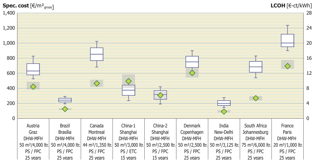
Figure 46: Specific Investment costs and levelized costs of solar thermal generated heat for large pumped domestic hot water systems
