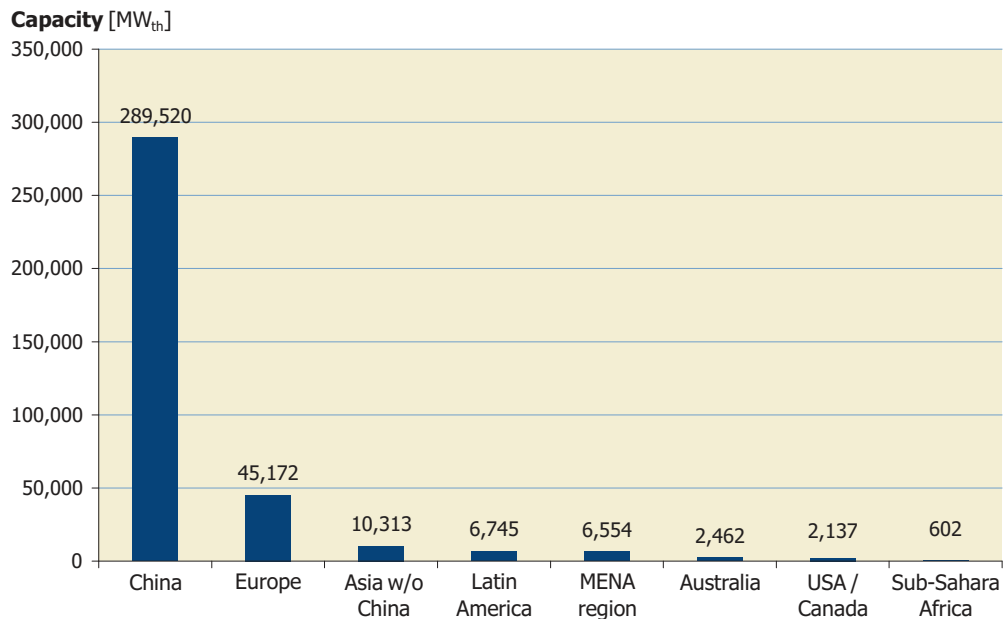
Figure 12: Total capacity of glazed flat plate and evacuated tube collectors in operation by economic region in 2014
