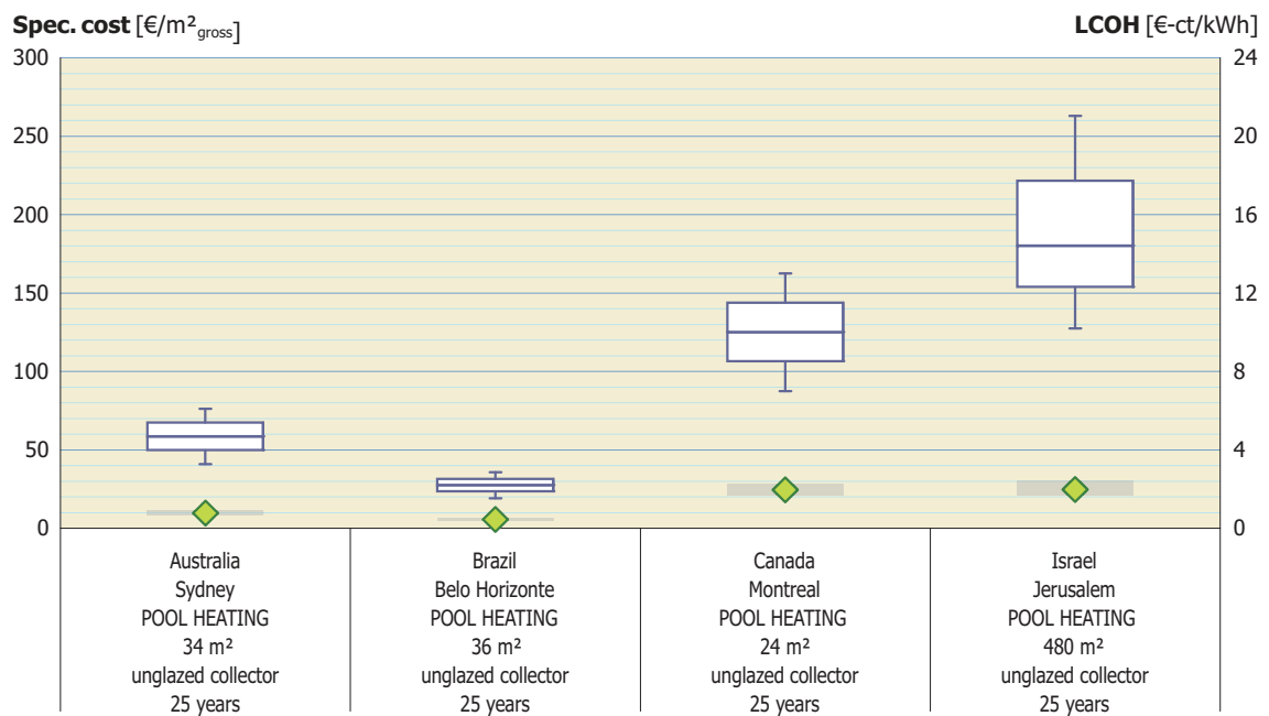
Figure 48: Specific Investment costs and levelized costs of solar thermal generated heat for swimming pool heating systems
